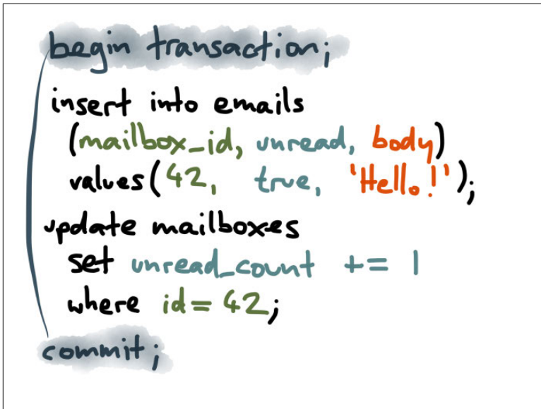
Figure 2-12. Transaction atomicity means that if you make several changes, they either all happen or none happen.
