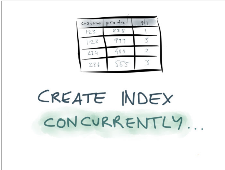
Figure 5-8. The CONCURRENTLY option in PostgreSQL allows an index to be built without locking the base table for writes.
